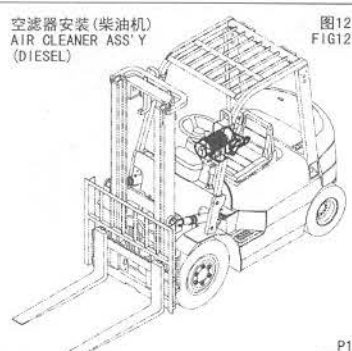
空滤器安装(柴油机) AIR CLEANER ASS'Y (DIESEL)
