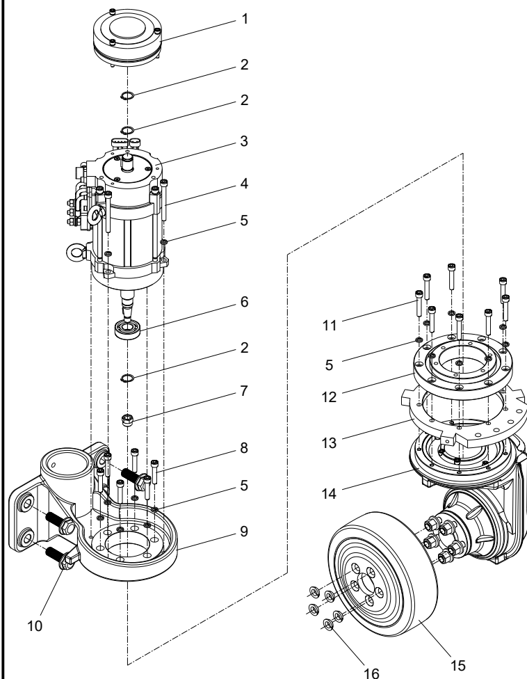
Fig.1 Driving system
