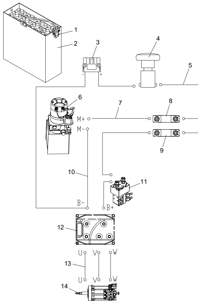
Fig.20 Wiring harness II
