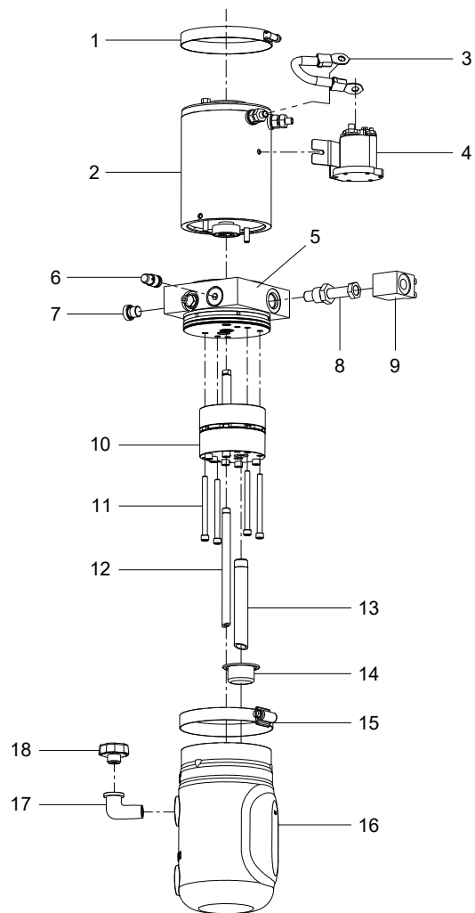
Fig.13 Hydraulic power unit
