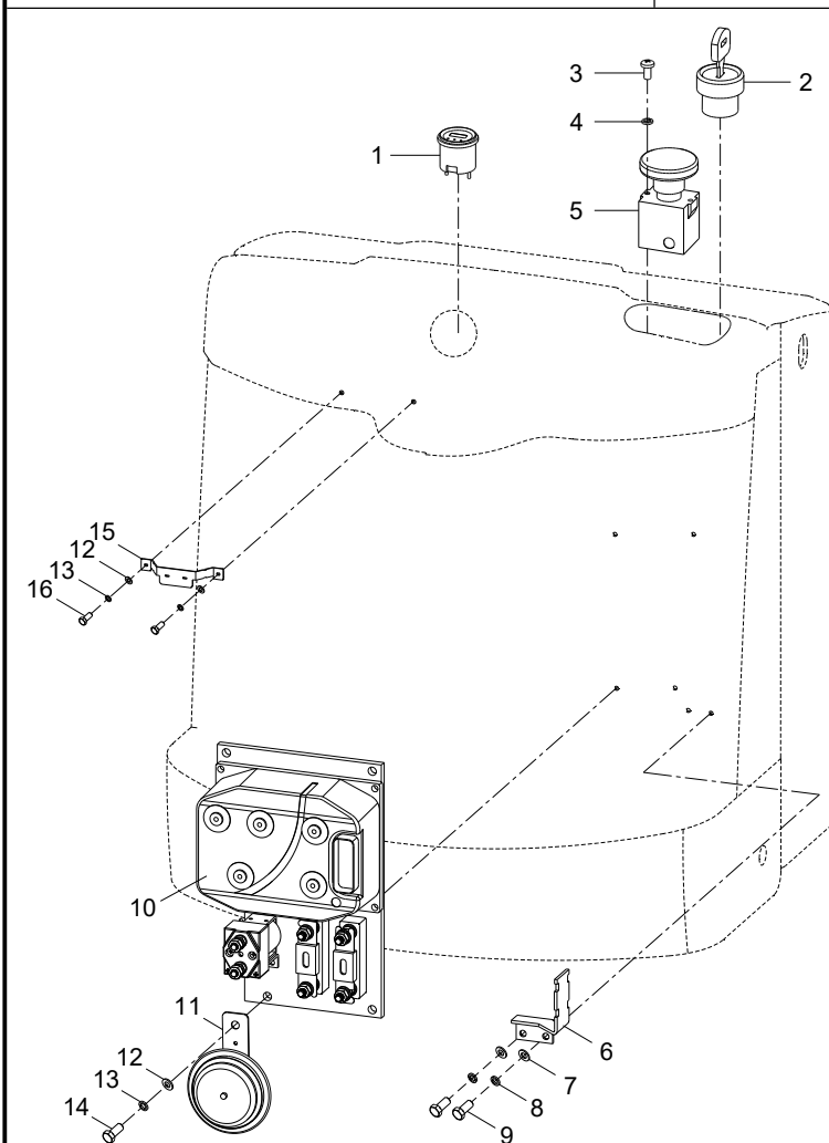
Fig.15 Electrical system I
