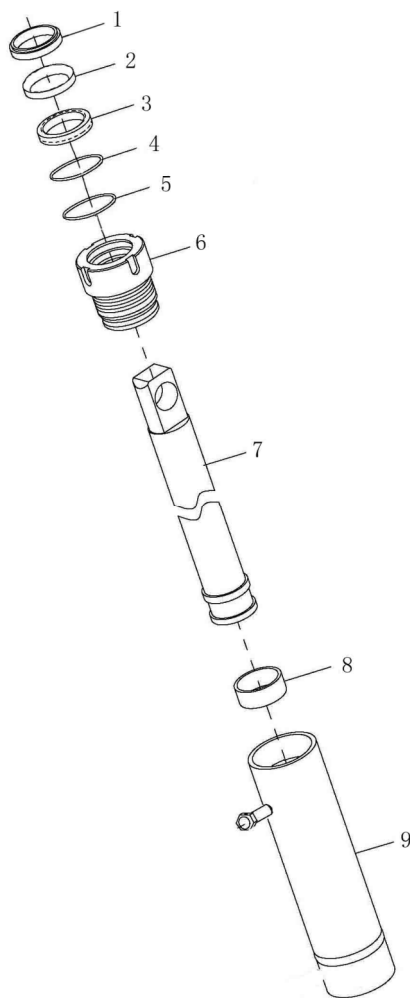
Fig.14 Lifting cylinder
