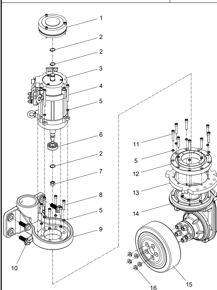
图 1 驱动系统 Fig.1 Driving system
