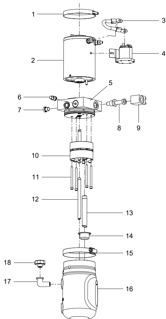
Fig.13 Hydraulic power unit
