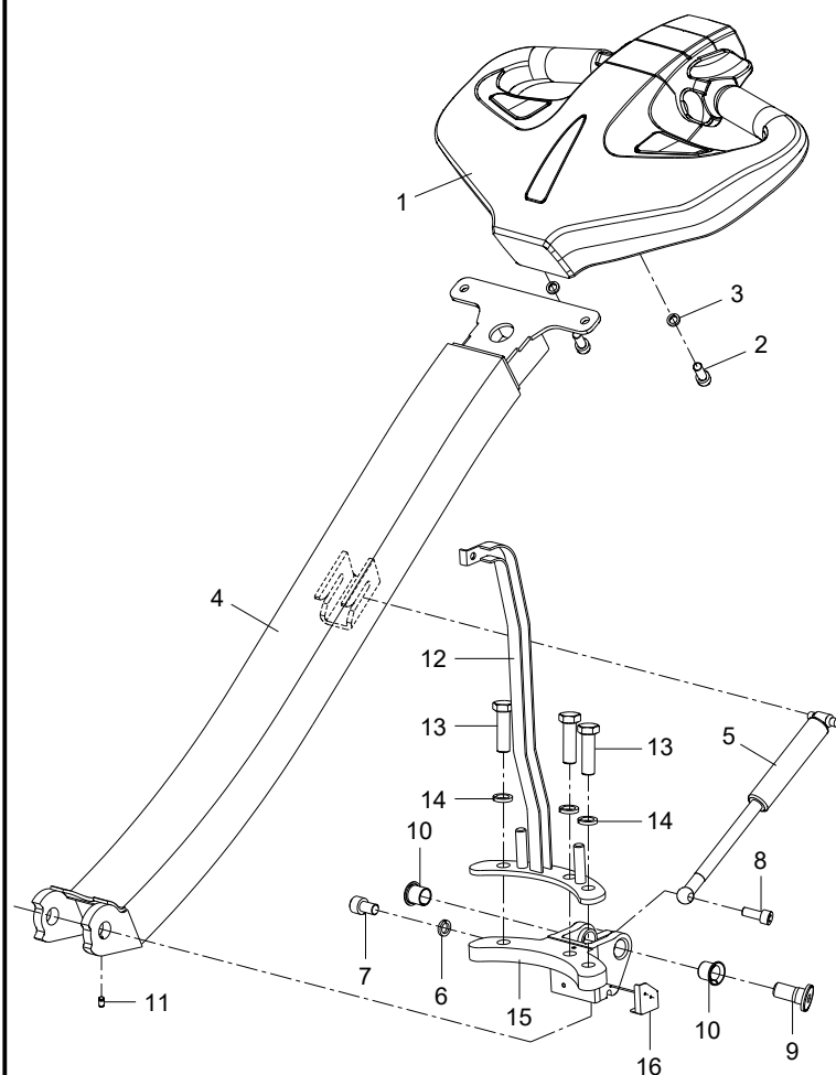
Fig.4 Steering control system
